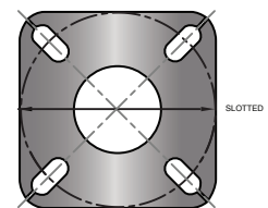
STL-1 TEMPLATE 10.00 X 10.00 X 0.75 ANCHOR PLATE 8.00" - 11.00" DIA. BOLT CIRCLE
